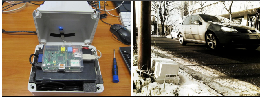
Fig. 1. The white box containing a raspberry-pi battery powered
